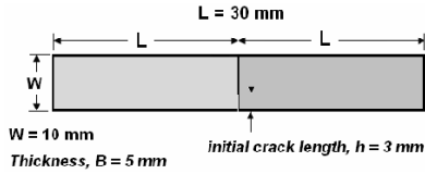
Fig. 1. Configuration of bone/cement bonded specimen for three-point bending test, h (=3\text{mm}) represents the initial length of interface crack.
